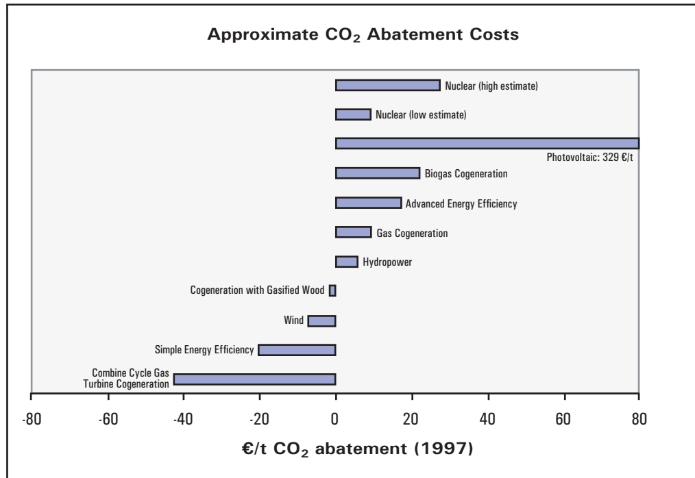
Figure 1: CO 2 abatement costs for various electricity systems (adapted from Öko Institute, 1997) Germany. The results are shown in figure 1.
